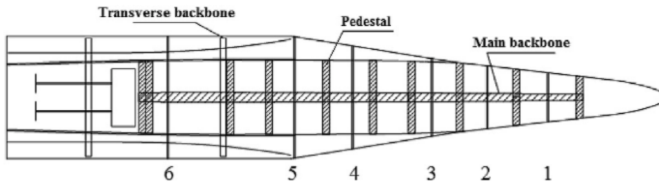
Fig. 4. A trimaran model featuring a longitudinal backbone and two transverse backbones [41].
