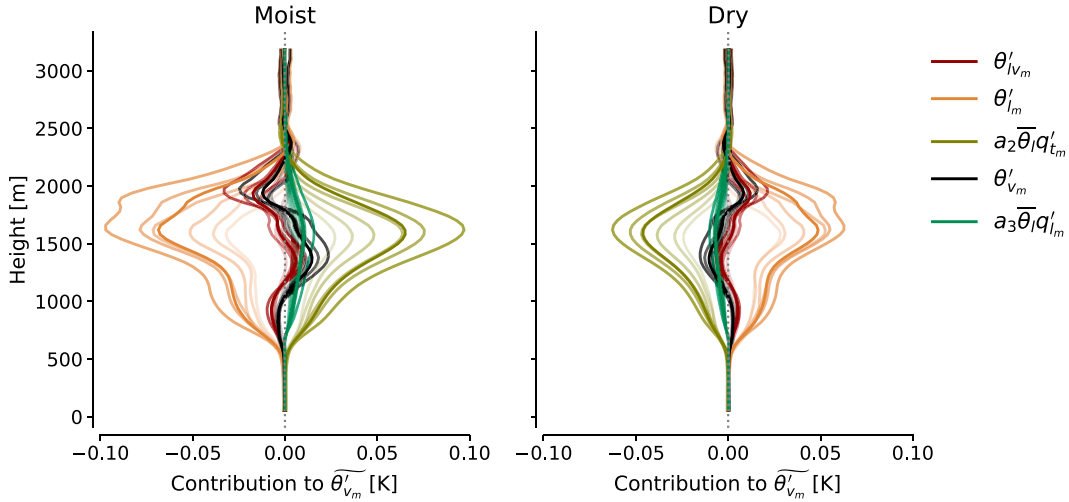
FIG. 9. Vertical profiles of \theta'_{vm} [Eq. (8)] and \theta'_{vm} [Eq. (12)], and their contributions from \theta'_m , q'_{tm} , and q'_{lm} , averaged over (left) moist and (right) dry mesoscale regions, over 10–16 h (dark lines) and over every hour between 10 and 16 h (transparent lines, in order of increasing opacity).
