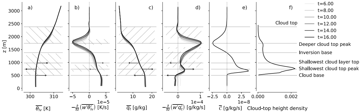
FIG. 17. Time evolution of vertical profiles of (a) \bar{\theta}_{lv} , (b) -(\partial/\partial z)(\overline{w' \theta'_{lv}}) , (c) \bar{q}_t , (d) -(\partial/\partial z)(\overline{w' q'_t}) , (e) \bar{C} , and (f) vertical distribution of cloud-top height throughout the simulation. Hatches indicate areas where (a), (c) \partial^2 \bar{q}_t / \partial \bar{\theta}_{lv}^2 > 0 , (b) \partial^3 \overline{w' \theta'_{lv}} / \partial z^3 < 0 , and (c) \partial^3 \overline{w' q'_t} / \partial z^3 < 0 at t = 16 h. Arrows emphasize the action of condensation and evaporation in very shallow clouds over the transition layer on the flux convergence terms and on the thermodynamic variables.
