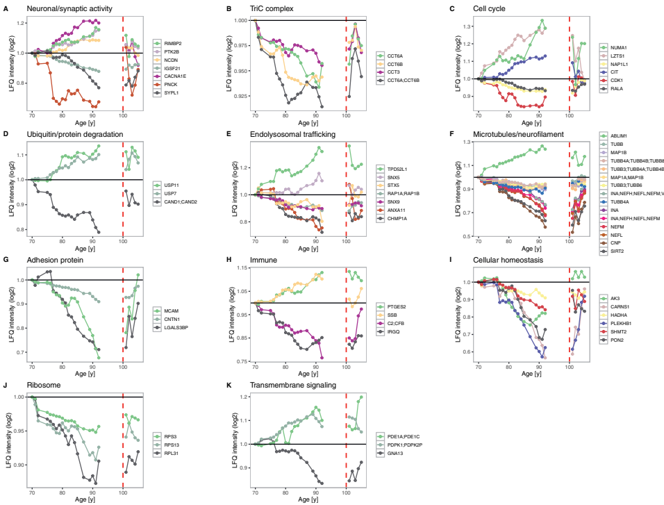
Figure 4.9: The smoothed protein abundance vs age in ND individuals and centenarians for CEN-Age proteins. For proteins belonging to each group the smoothed protein abundances (Methods) for ND individuals and centenarians is plotted versus age. The vertical red dashed line indicates the abundance in the age continuum until 100 years, and abundance levels measured in centenarians.
