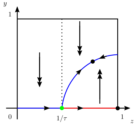
Fig. 5 Stability of the branches of the critical manifold C_0 of (17). Blue: stable; red: unstable. Green dot: non-hyperbolic point; black dots: equilibria. Double arrows: fast flow; single arrows: slow flow. (Color figure online)
