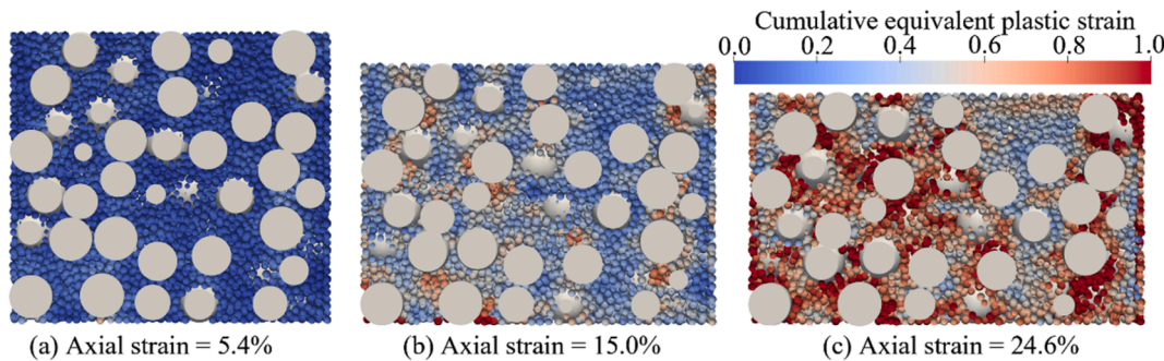
Fig. 23. The plastic zone of 1:5 particle size ratio sample under 60% coarse particle content.
