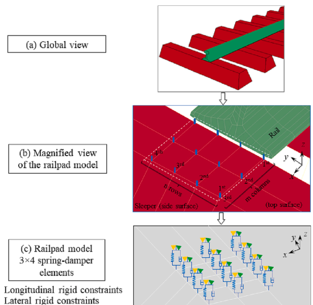
Fig. 4. Fastening model for corrugation consistent initiation and growth.
