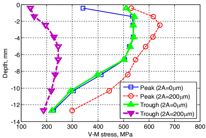
Fig. 10. The maximum V-M stress distribution in rail depth at corrugation peak and trough under 2A_{\max} = 0 and 200 \mu\text{m} respectively (Element 682,718 corresponds to corrugation peak, and element 682,700 corresponds to corrugation trough).
