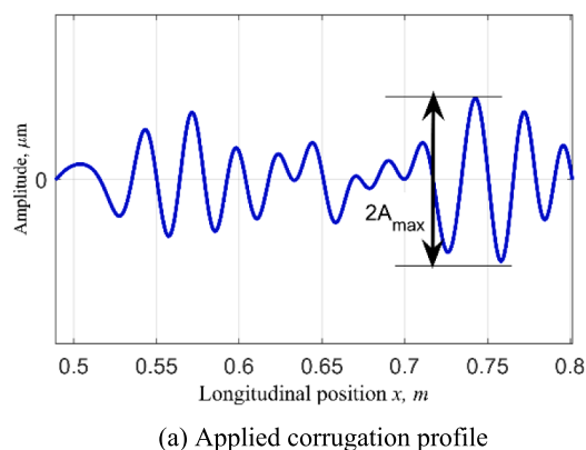
Fig. 7. Corrugation profile applied in the model.
