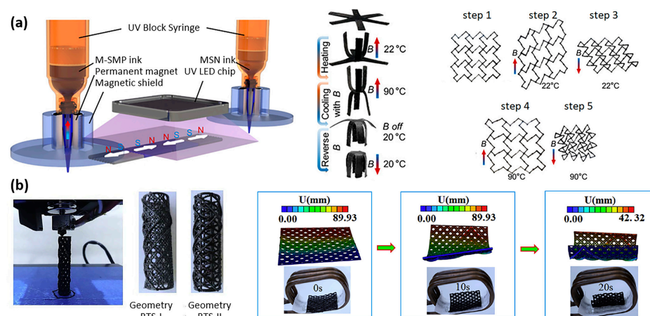
Figure 6. The 3D-printed shape-memory magnetic polymer composites and 3D printing of magnetic shape-memory polymers. (a) Multimaterial 3D printing technology for magnetic soft composites and magnetic shape-memory polymers. Left: 3D printer schematic. Middle: shape transformation. Right: active metamaterial. Initial shape (step 1), deformed shapes at 22 °C under upward (step 2) and downward (step 3) magnetic fields. Deformed shapes at 90 °C under upward (step 4) and downward (step 5) magnetic fields (reproduced with permission from Applied Materials & Interfaces, ACS) [49]. (b) The 3D printing of magnetic shape-memory polymer composites made of polylactic acid (PLA) and \text{Fe}_3\text{O}_4 , to fabricate personalized tracheal scaffolds. Left: 3D printing process at 180 °C. Right: wireless actuation (reproduced with permission from Composites Science and Technology, Elsevier) [50,51].
