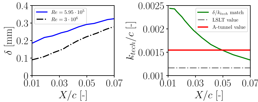
FIGURE 3 On the left, the boundary layer thickness from k - \omega - SST calculations corresponding to the Re of the A-tunnel experiments (blue solid line) and of the LSLT experiments (black dashed-dotted line) are shown. On the right, the gray-dashed-dotted line shows the k_{tech}/c value used in the LSLT measurements. The green line refers to the k_{tech}/c value computed to provide the same \delta/k_{tech} as in the LSLT measurements. The red line refers to the final value employed in this study.
