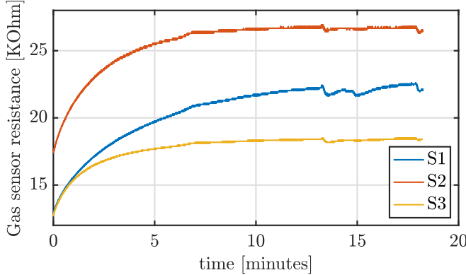
Fig. 5: Power up of the three gas sensors mounted on the tip of the soft robot. Note that each sensor reaches a different resistance baseline in about the same amount of time.
