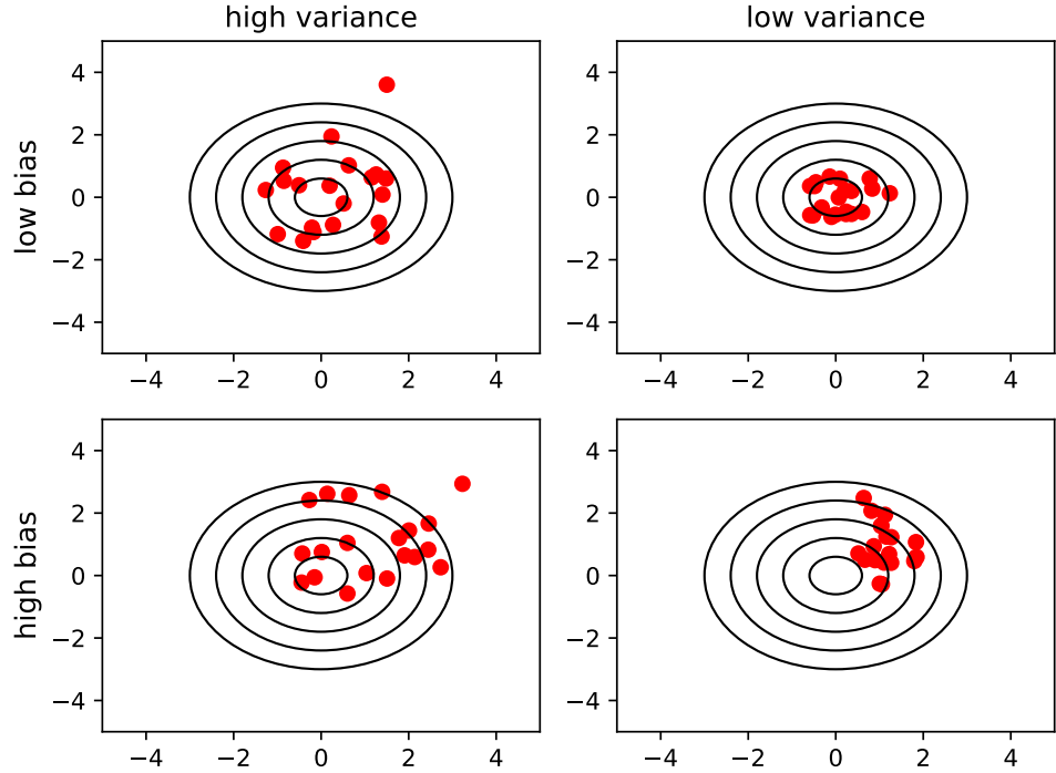
Figure 1.1: Illustration of bias, variance and accuracy
