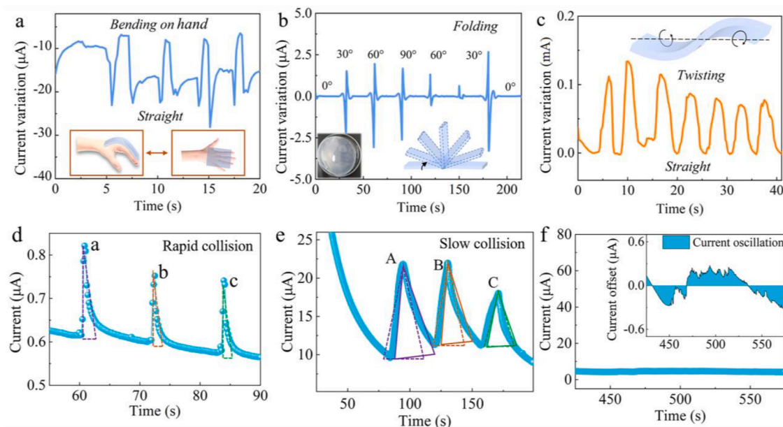
Fig. 5. Responses to bending (a), folding (b), twisting (c), rapid collision (d), slow collision (e) and heat producer (f) of the -H-C-L-A-H device. The folding angles are 0°, 30°, 60°, 90°, 60°, 30° and 0° respectively. And the illustration is the sample used in the actual test. The thickness of each gel round piece was 2 mm (a-c). During the rapid collision, pressures were applied at points a, b and c respectively, and the right-angled triangle models are used to represent relationships between pressure and current variation (d). During the slow collision, pressures were applied at points A, B and C respectively, and the isosceles triangle models are used to describe relationships between pressure and current variation (e). A heat producer is a hot-water bag and the illustration is the current-oscillation relationship (f).
