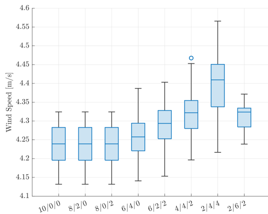
Figure A2. Average wind speeds downstream for different wake zones. The numbers on the x axis indicate the unit length of measure for wake zone 1/2/3 respectively. The 25th, 50th, and 75th percentile are shown as a box. The bars indicate the distance to the, non-outlier, minima and maxima in the data set. Any circles indicate data outliers excluded in the boxplot.
