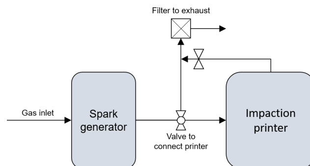
Figure 2. Schematic of the spark ablation and printer setup showing all gas inlets and outlets.
