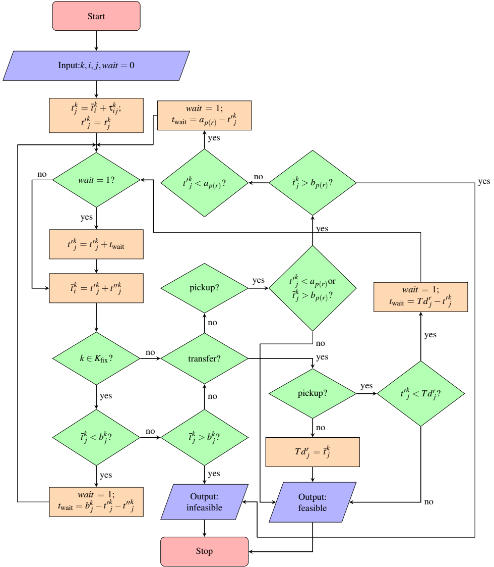
Figure A.1: Barge and train's time at pickup/delivery/transshipment terminal in ALNS
