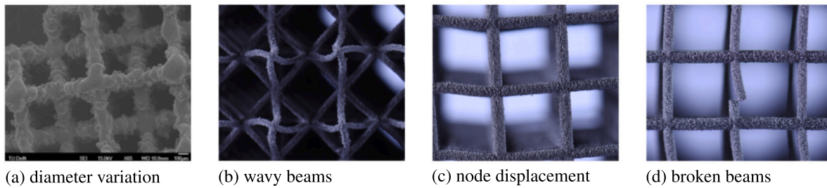
Fig. 1. Four types of imperfections are presented that commonly appear during the fabrication process. Subfigure (a) is reprinted by permission from Elsevier [6]. Figures (b)–(d) fabricated with selective laser sintering (SLS) on a Sintratec S1 printer.
