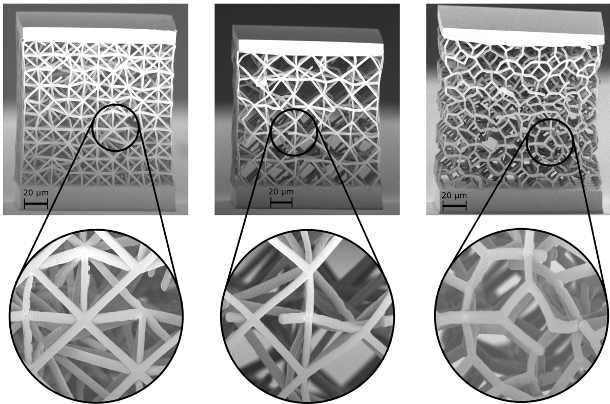
Fig. 19. Fabricated octet, octahedron, and bitruncated octahedron samples (from left to right) with deliberately introduced imperfections satisfying the distributions \xi_{\text{nds}} = 0.238 , \xi_{\text{mis}} = 0.157 , \xi_{\text{wvy}} = 0.054 , and \xi_{\text{dia}} = 0.113 .
