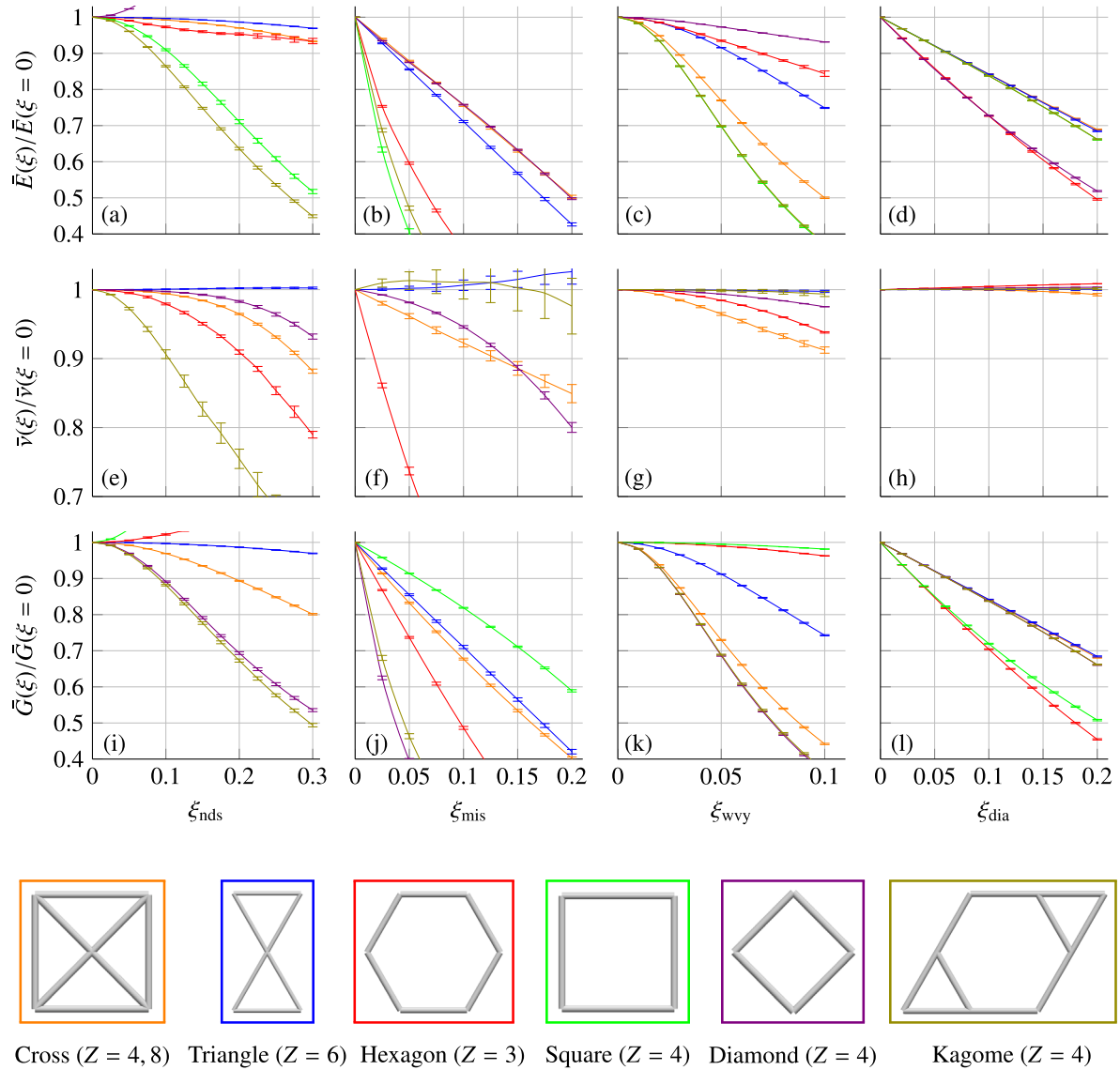
Fig. 5. Sensitivity of 2D bending- and stretching-dominated truss topologies with respect to the imperfection standard deviations \xi_{\text{nds}} , \xi_{\text{wvy}} , \xi_{\text{dia}} , and missing beam probability \xi_{\text{mis}} . Each error bar represents the standard deviation obtained from N = 100 random realizations of the imperfect trusses. Line and marker colors correspond to the six truss topologies shown below. While all nodes in any of the structures have the same coordination number of connecting struts, Z , the cross unit cell has two type of nodes, connected to different numbers of struts, which is why the coordination number for some nodes in the cross lattice is Z = 4 , while for others Z = 8 . (For interpretation of the references to color in this figure legend, the reader is referred to the web version of this article.)
