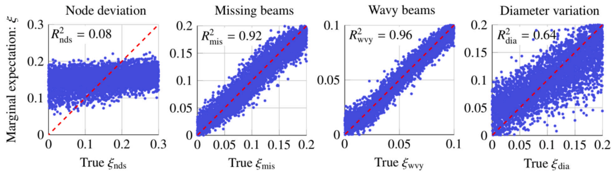
Fig. 18. Accuracy of predicted marginal expectation of each imperfection vs. the true value on the test dataset, using the uniaxial Young's moduli of three 3D truss topologies (octet, bitruncated octahedron, octahedron) as input parameters. Due to the smaller number of input parameters (number of mechanical properties and number of UCs), the accuracy of the prediction decreases when compared to Fig. 15. All dashed lines (in red) represent the ideal line with zero intercept and unit slope; the corresponding R^2 deviations are indicated.
