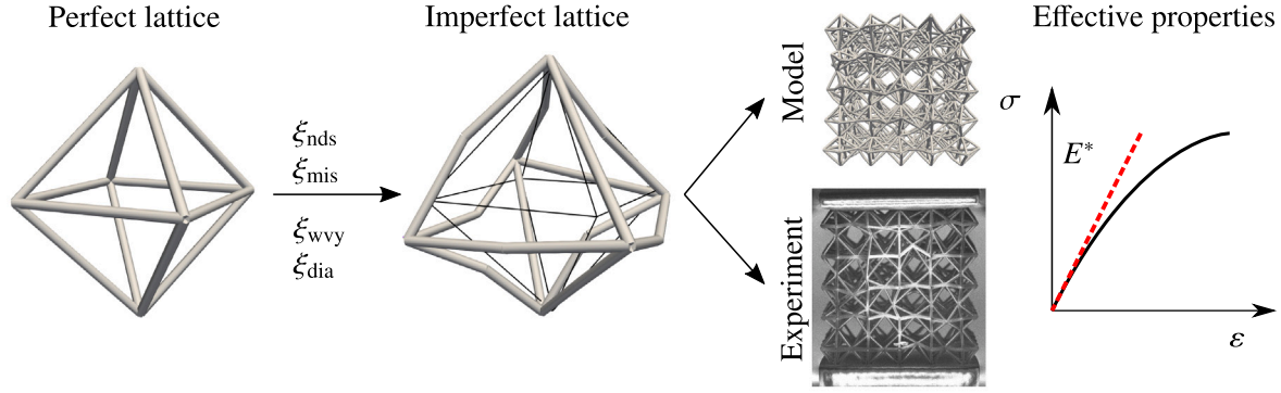
Fig. 9. Protocol for comparing simulated with experimentally determined stiffness data: after applying imperfections to a defect-free lattice, the effective response of the truss is obtained from the stress–strain curve under uniaxial compression—both from simulations and from experiments on a 3D-printed truss.
