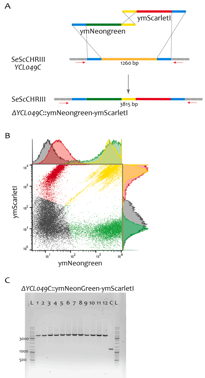
Fig. 8. Genomic integration into landing site SeYCL049C of two in vivo assembled DNA fragments expressing ymNeongreen and ScarletI. A) Schematic overview of the genomic integration strategy for in vivo assembly of ymNeongreen and ScarletI DNA fragments. B) Fluorescent profile the transformed population when aiming for integration of two fluorescent expression cassettes. The fluorescence corresponding to ymNeongreen and ymScarlet is plotted for 100,000 events. Flow cytometry was performed for three biological replicates; one representative replicate is shown. C) Genotyping of the sorted ymNeongreen + Scarlet + single colony isolates.
