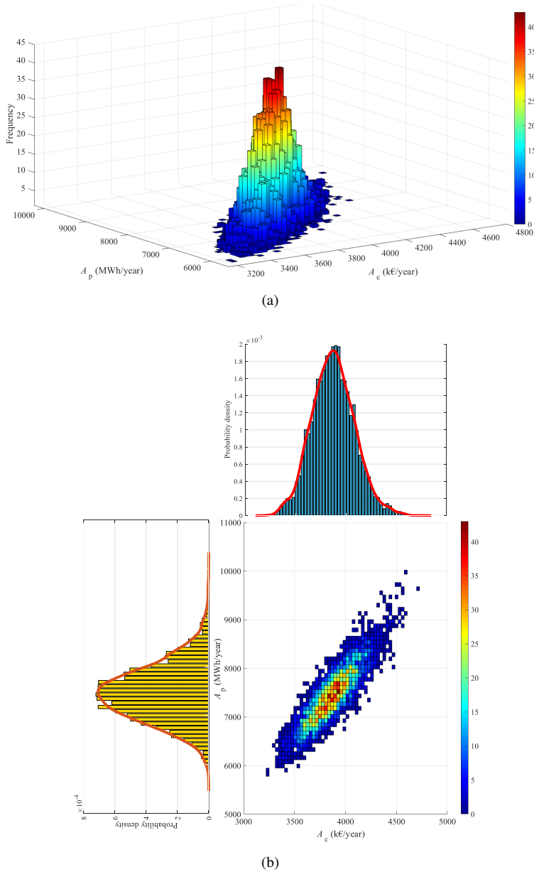
Figure 4.13: Distribution of the derived results: (a) Bivariate histogram plot. (b) Plot with marginal probability density function
