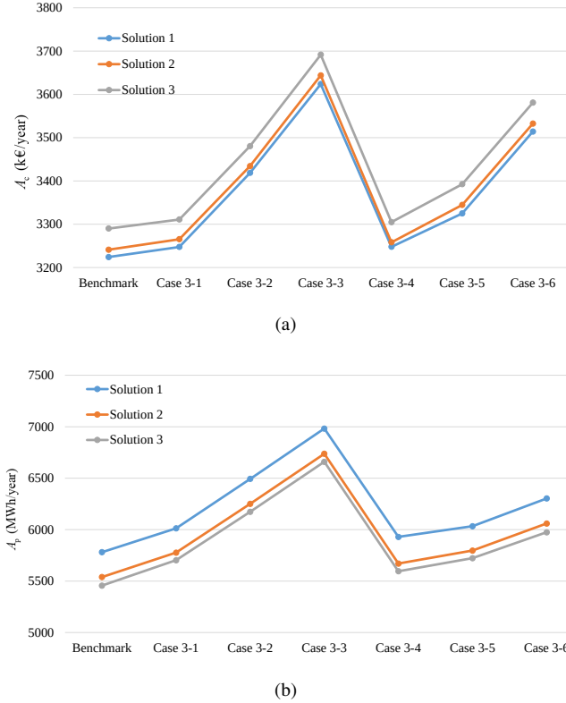
Figure 4.10: Comparison of Cases 3-1 to 3-6: (a) Maintenance cost. (b) Production loss
