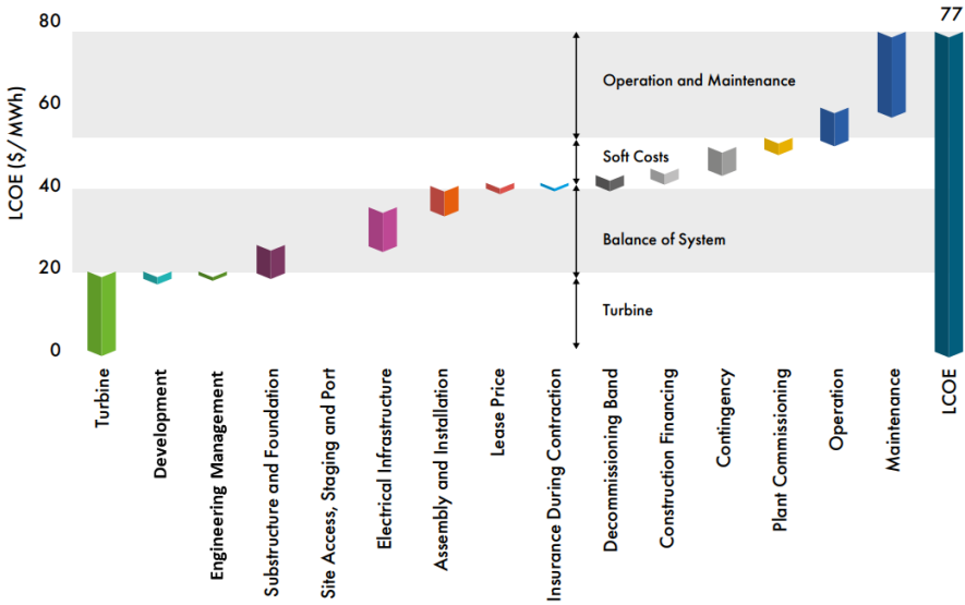
Figure 1.4: LCOE breakdown for typical fixed-bottom offshore wind farm [64]
