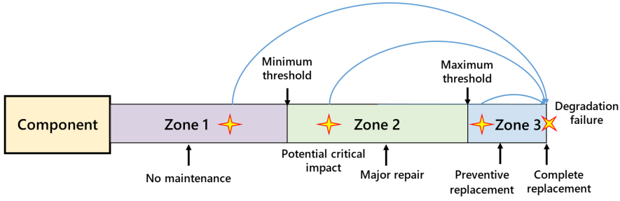
Figure 3.4: Maintenance actions for the components of different stages
