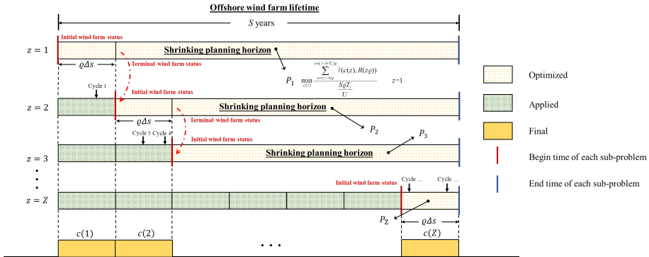
Figure 7.2: Schematic representation of the shrinking planning horizon over the wind farm lifetime
