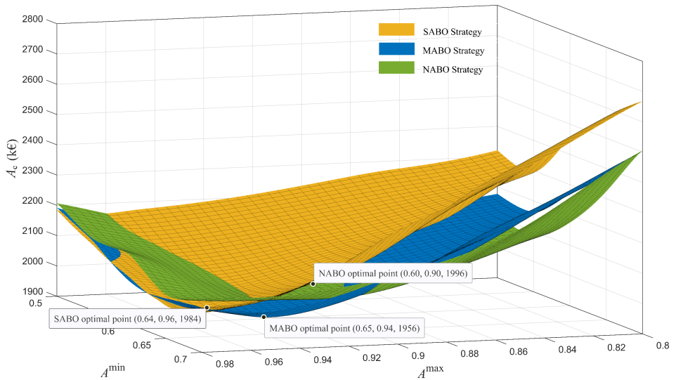
Figure 3.10: Annual cost with different age threshold under three strategies
