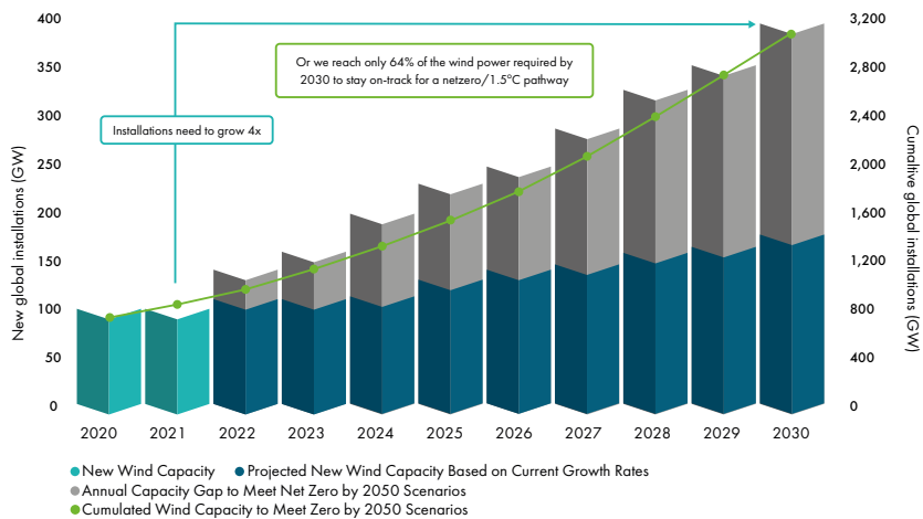
Figure 1.1: Lagging growth leads to wind energy shortfalls in this decade [64]
