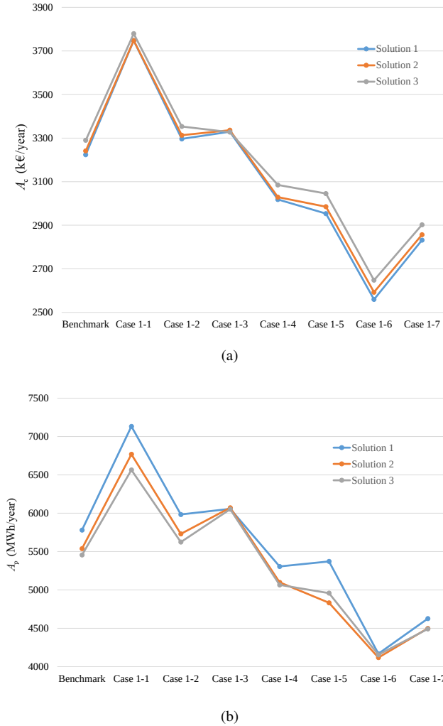
Figure 4.7: Comparison of Cases 1-1 to 1-7: (a) Maintenance cost (b) Production loss
