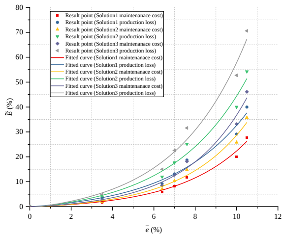
Figure 4.9: Average prediction error \bar{e} versus maintenance performance
