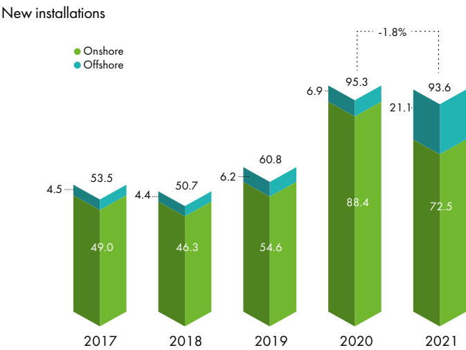
Figure 1.2: Global new installation [64]
