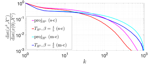
Fig. 3. Trajectories of \text{dist}(\mathbf{x}^k, \mathcal{X}^*) / \text{dist}(\mathbf{x}^0, \mathcal{X}^*) for distributed bilateral negotiation with operators \text{proj}_{H^k} and T_{H^k} := (1 - \beta)\text{proj}_{H^k}(\cdot) + \beta \text{overproj}_{H^k}(\cdot) for single-contract (s-c) and multi-contract (m-c) market setups.
