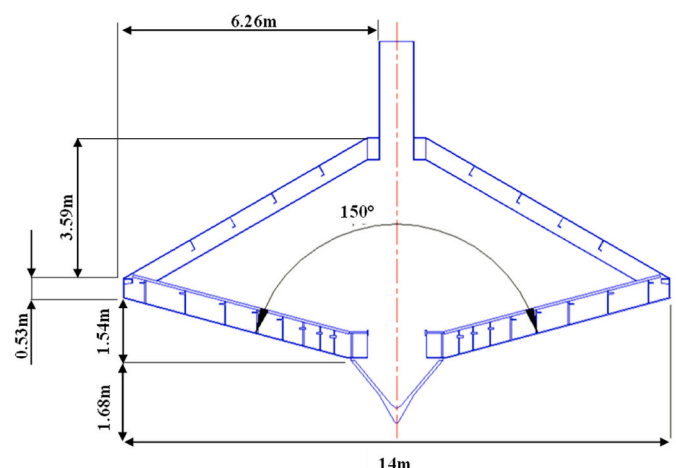
Fig. 1. Spudcan geometry.
