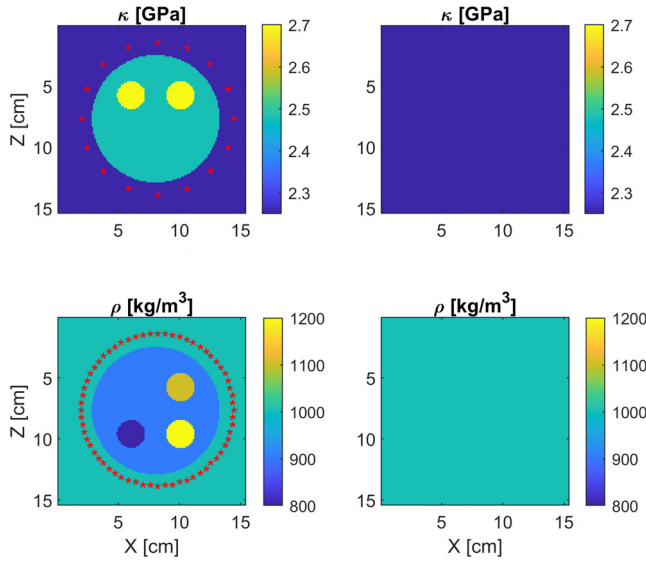
FIG. 13. (Color online) Ultrasonic model designed to investigate the effects of multi-parameter cross talk on the inversion results. The left and right columns of panels show the true model and the initial model, respectively. The locations of the receivers and sources are indicated on the true bulk modulus and mass density models, respectively. The excitation profile used in this numerical experiment is shown in Fig. 7.
