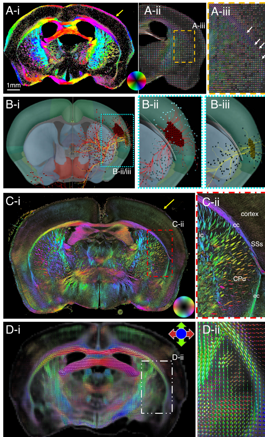
Fig. 3. Fiber orientations in the mouse brain. (A) SAXS-based fiber orientation map of a 25 µm-thick section where the fiber orientation is color-encoded according to the color wheel with 4 quadrants per pixel as described in Section 2.3 (A-i), or with orientation-encoded colored bars (A-ii). To facilitate viewing of the image (A-ii), fiber orientations from each 5×5 pixel set are averaged. (A-iii) Expanded view of orange boxed region in (A-ii), where fibers spreading from the internal capsule through the caudoputamen cross the corpus callosum and external capsule (white arrows) to extend radially into the cortex. In addition, cortical radial fibers reach the outermost molecular layer of the cortex and cross with the circumferential myelinated fibers along the brain surface (yellow arrow in A-i). (B) Visualization of the Allen Mouse Brain Connectivity Atlas experiments 297945448-SSs (B-i) and 520728084-SSs (B-ii) ( https://connectivity.brain-map.org/projection/experiment/297945448 and https://connectivity.brain-map.org/projection/experiment/520728084 ), which included injections in the supplemental somatosensory area, showing axons in red and yellow colors respectively from a C57BL/6J mouse tagged with green fluorescent protein. (B-i) Posterior view of the two experiments. (B-ii/B-iii) Enlarged view of the cyan box in (B-i), with the corpus callosum 3D rendered in semi-transparent gray color to enable visualization of the crossing cortical-caudoputamen fibers. Images generated using the Atlas' 3D viewer ( https://connectivity.brain-map.org/3d-viewer ). (C) 3D-PLI image showing fiber orientations in a 60 µm-thick mouse brain section, at a plane ~300 µm anterior compared to the section in (A). C-ii is an enlarged view of the red-boxed area in C-i. Yellow arrow points to molecular layer of cortex. (D) Diffusion MRI-derived fiber orientation maps from same mouse and same virtual section as in (A). Fiber orientation distributions are represented by a set of spherical harmonics, allowing multiple fibers per voxel, and are color-encoded according to arrows in top right of (D-i). (D-ii) Enlarged view of white box in D-i, showing no distinguishable corpus callosum crossings. cc: corpus callosum, ic: internal capsule, ec: external capsule, CPu: caudoputamen, SSs: supplemental somatosensory area.
