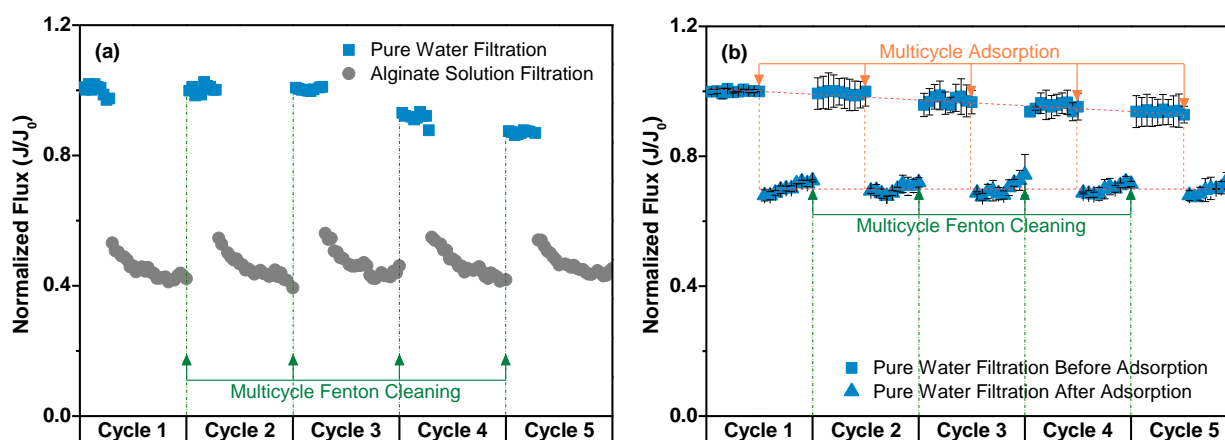
Figure 4.7 Multiple-cycle (a) filtration ( J_0 = 39.5 \text{ L m}^{-2} \text{ h}^{-1} ) and (b) adsorption with alginate solutions and periodical Fenton cleaning ( [\text{H}_2\text{O}_2]_0 = 30.0 \text{ mM} , \text{pH} = 3.3 ) using an FeOCl pre-coated membrane.
