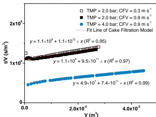
Figure S4.3 t/V vs. V profiles of pristine ceramic NF membrane operated at TMP = 2.0 or 4.0 bar and CFV = 0.3 or 0.9 m s -1 . The straight lines correspond to the linear fitting of t/V vs. V profiles to the cake filtration model.
