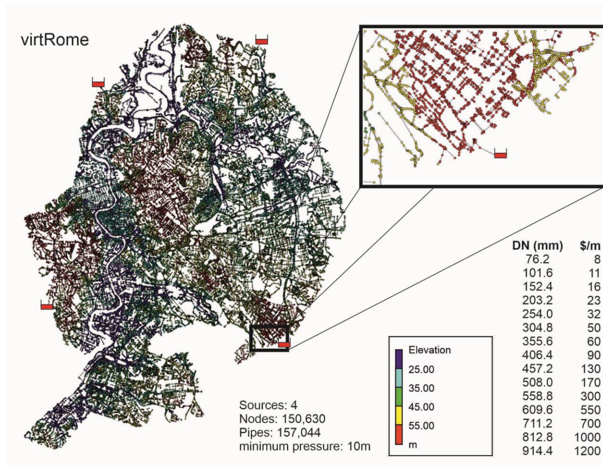
Figure 4. The layout of the virtRome case study
