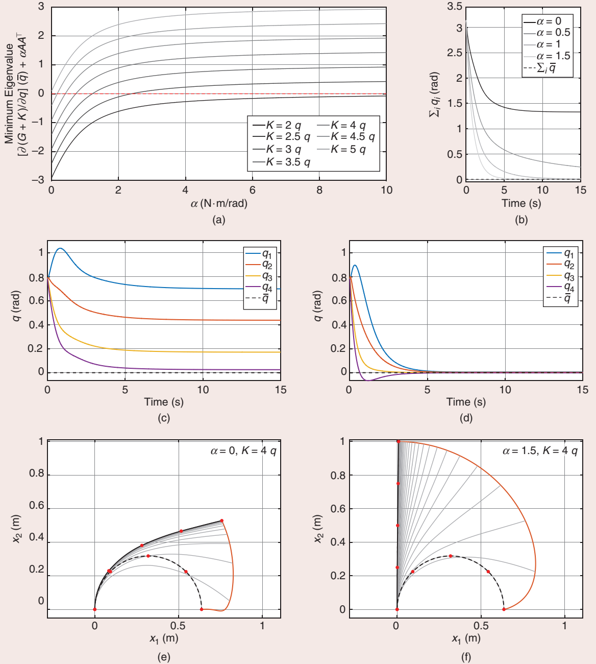
FIGURE 10 Examples of (33) controlling a slender planar soft segment actuated through a torque at its tip. The robot is modeled with four CC segments ( n = 4 ) of equal mass ( m = 0.25 Kg), length ( L = 0.25 m), and homogeneous impedance ( K(q) = 4q , D(q)\dot{q} = 1.2\dot{q} ). Gravity is pointing downward ( \phi = \pi ). We aim for stabilizing the robot's straight configuration \bar{q} = [0, 0, 0, 0]^T rad. (a) Changing the gain \alpha and the stiffness K affects the stability, measured as the minimum eigenvalue of (32). The red dashed line highlights the threshold above which the robot is locally stable. Closed-loop evolutions appear in (b)–(f). (b) The evolution of A^T q for different choices of \alpha and \beta = 1 (N · ms/rad). The gains are (\alpha, \beta) = (0 (N · m/rad), 1 (N · ms/rad)) in (c) and (e) and (\alpha, \beta) = (0 (N · m/rad), 1 (N · ms/rad)) in (d) and (f). The robot starts at rest from the configuration q(0) = [\pi/4, \pi/4, \pi/4, \pi/4]^T rad. (c) and (d) The evolution in time of the four curvatures. (e) and (f) The evolution of the robot's shape. The initial condition is a black dashed line, the final condition is a black solid line, and the ends of the segments are highlighted with red dots.
