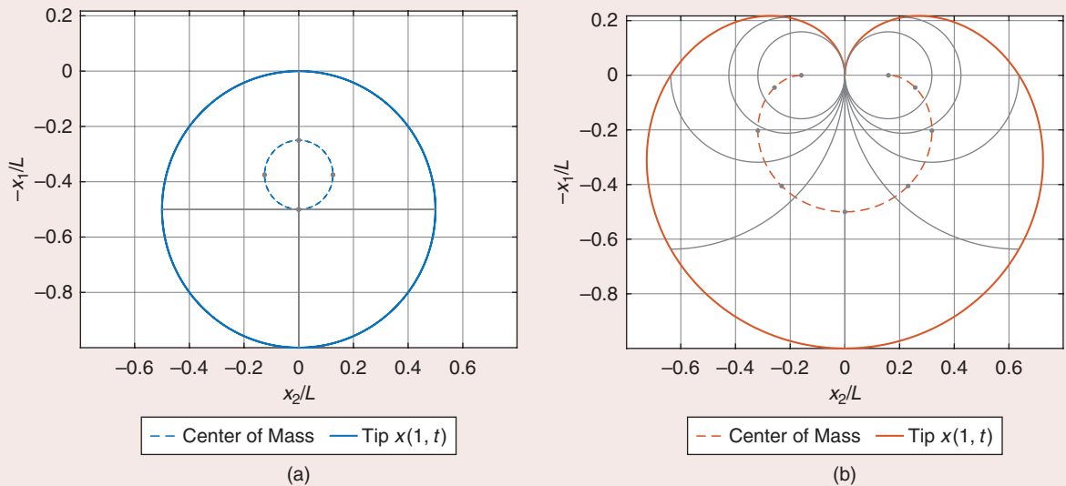
FIGURE S2 The geometrical characterization of (a) a rigid robot with a single revolute joint and (b) a CC robot. The behaviors are similar to the straight configuration, but they strongly depart from one another when the angle |q| increases. The configurations corresponding to q \in \{-2\pi, -3\pi/2, \dots, 3\pi/2, 2\pi\} are shown with thin gray lines. The corresponding centers of mass are also reported as gray dots. Note that this range of angles corresponds to two full rotations for the rigid links case.
