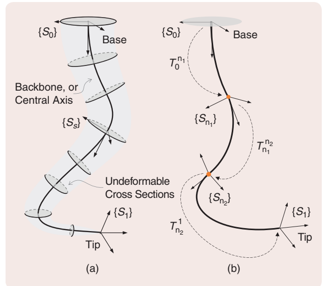
FIGURE 1 (a) A soft robot as described within rod theories. The central axis, or backbone, is a spatial curve that can deform. Cross sections are assumed to be undeformable, and they are rigidly connected to the curve. Some examples of disk-like cross sections are highlighted in the figure. To each point is also attached a reference frame \{S_s\} , where s is the normalized arc length. (b) Piecewise constant strain models with three segments. First, four nodes along the backbone are identified (0, n_1, n_2, 1) . Then, the associated transformation matrices (T_0^{n_1}, T_{n_1}^{n_2}, T_{n_2}^1) are parameterized by a finite set of variables. The robot configuration q is defined as the collection of these variables. In piecewise constant curvature models, two subsequent nodes are always connected by an arc of a circle.
