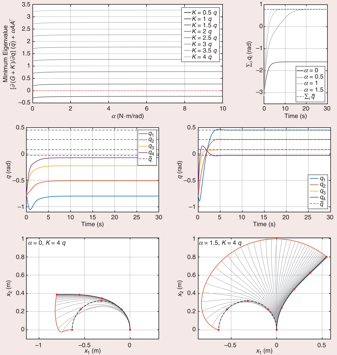
FIGURE 11 Examples of (33) controlling a slender planar soft segment actuated through a torque at its tip. Everything is as in Figure 10 except for the initial and desired configurations, which are q(0) = [-\pi/4, -\pi/4, -\pi/4, -\pi/4]^\top rad and \bar{q} = [0.4413, 0.2720, 0.0872, -0.0179]^\top rad, respectively. The latter is such that \sum_i \bar{q}_i = \pi/4 . Note that even if \alpha = 0 results in local asymptotic stability of \bar{q} [see (a)], it is not sufficient to enlarge the region of asymptotic stability enough to include q(0) .
