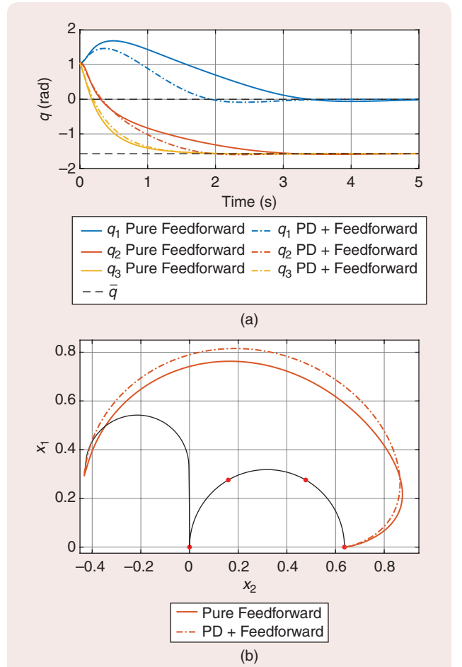
FIGURE 7 The pure feedforward controller (15) and the PD with feedforward controller (23), regulating the shape of a planar soft robot. (a) The evolution of configurations in time. (b) The evolution of the tip in space. The robot shape is described by three CC segments, each independently actuated (that is, A = I ). The segments are 0.33 m long and 0.33 Kg heavy. Gravity is aligned with the base, and it points downward. The elastic forces and dissipative forces are K(q) = q and D(q) = q/3 . The initial condition is q(0) = (\pi/3, \pi/3, \pi/3) and \dot{q} = 0 . The desired configuration is \bar{q} = (0, -\pi/2, -\pi/2) . Both corresponding shapes in the bottom plot are shown as solid black lines. The initial shape also has red dots marking each segment's beginning and end. The control gains are \alpha = I and \beta = I/2 .
