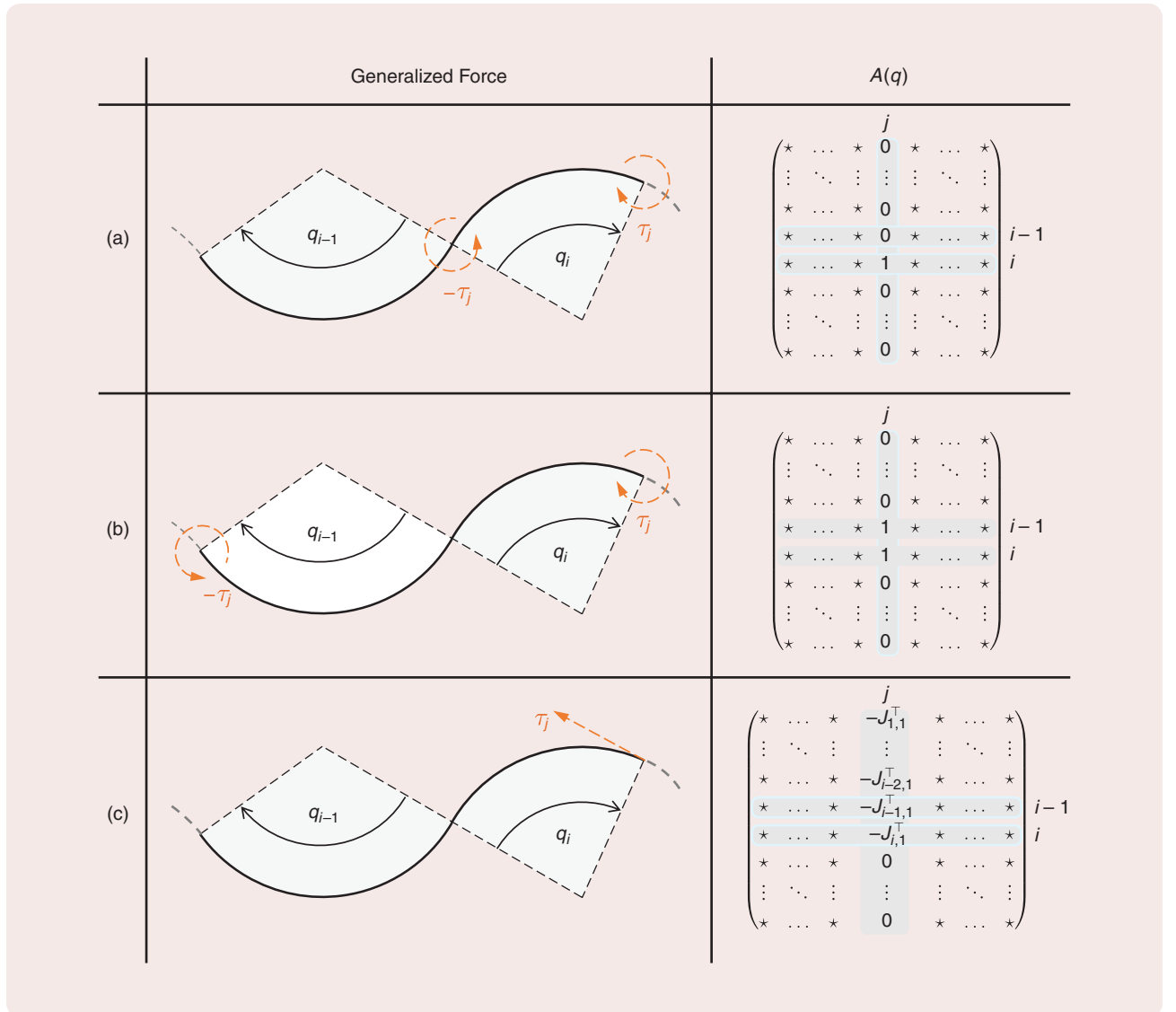
FIGURE 3 Actuation patterns resulting in different elements of the matrix A(q) . The examples are focused on how a generalized force \tau_j that is applied to the j th segment is mapped in the configuration space. CC discretization is used for illustrative purposes. One actuated segment is represented with one or two CC segments: (a) coarse internal discretization and (b) finer internal discretization. The actuator produces an internal pair of opposite torques. This is the case of a pair of pressurized chambers and of a tendon-driven system with motors placed at the base of the segment. (c) \tau_j is a force applied tangentially to the tip of the i th segment. Here, J_{k,1} is the k th element of the Jacobian mapping \dot{q} in the first linear velocity of the tip of segment i .
