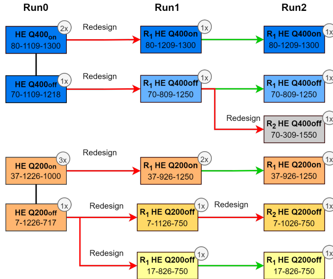
(b) Technology sensitivity study - Battery specific energy 700Wh/kg
