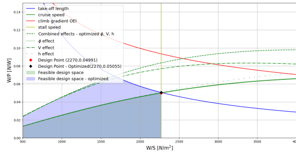
Fig. 19 Climate-optimized aircraft-level power-loading diagram
