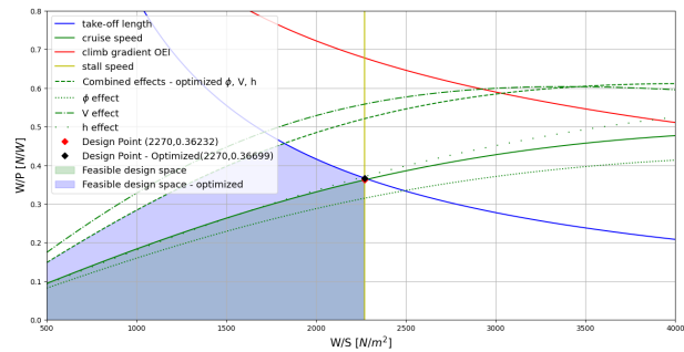
Fig. 21 Climate-optimized Electric Motor power-loading diagram
