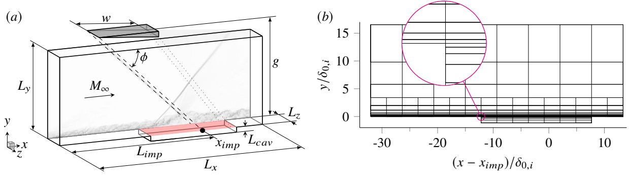
Fig. 1 (a) Schematics of the computational domain, and (b) block distribution of the computational grid.
