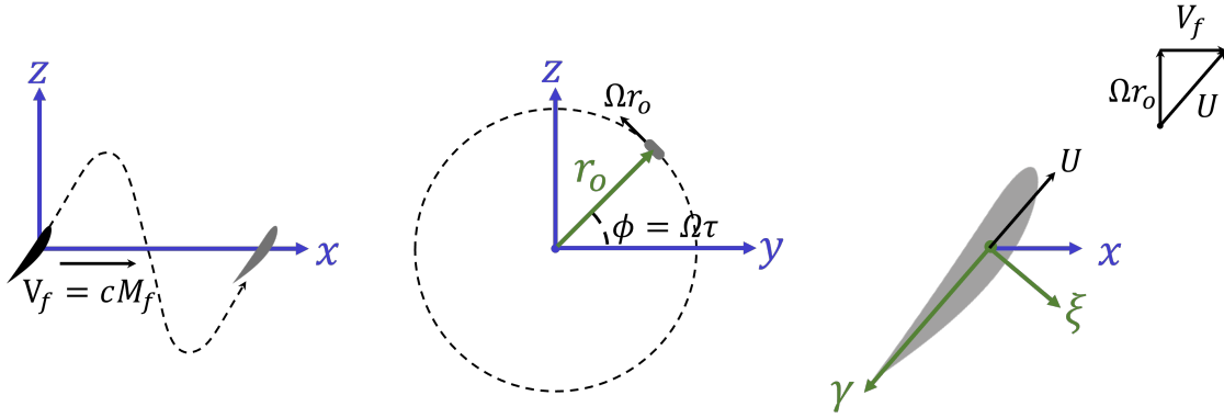
Fig. 1 Helical and Cartesian coordinate systems (adapted from Ref. [19]).
