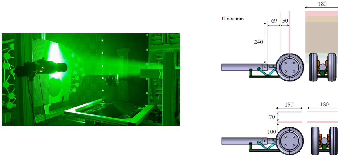
Fig. 6 PIV setup and measurement planes. Distances in mm.
