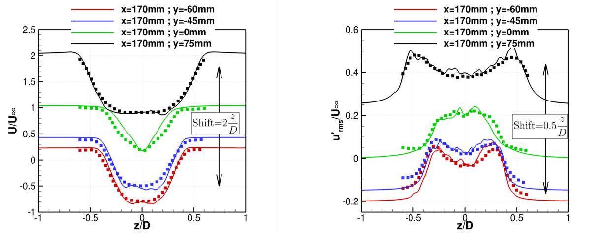
Fig. 12 Mean and RMS velocity profiles at x = 170\text{mm} ( x/D = 1.13 ) for the baseline configuration. Left: mean streamwise velocity u ; Right: streamwise RMS velocity fluctuations u' . Symbols: experiment; solid lines: ZDES simulation.
