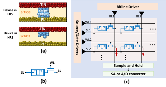
Fig. 1: (a) ReRAM memristor device behavior (b) 1T1R memristor cell (c) CIM tile encompassing crossbar and peripherals
