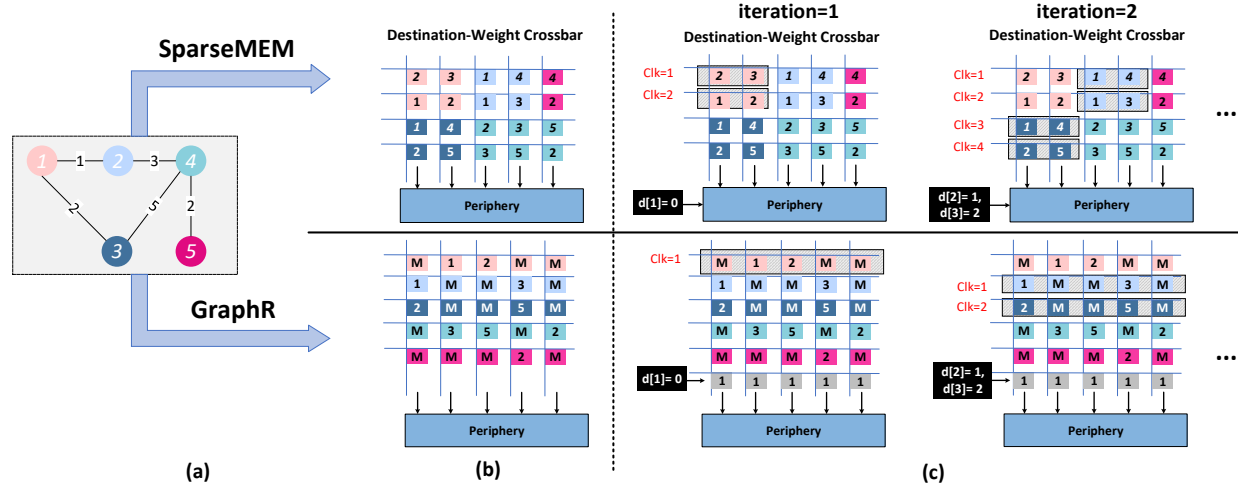
Fig. 4: (a) Graph example; (b) mapping of graph information into crossbar for computation phase considering SparseMEM and GraphR design; (c) the first two iterations of the SSSP algorithm starting with source vertex 1. “M” means no connection
