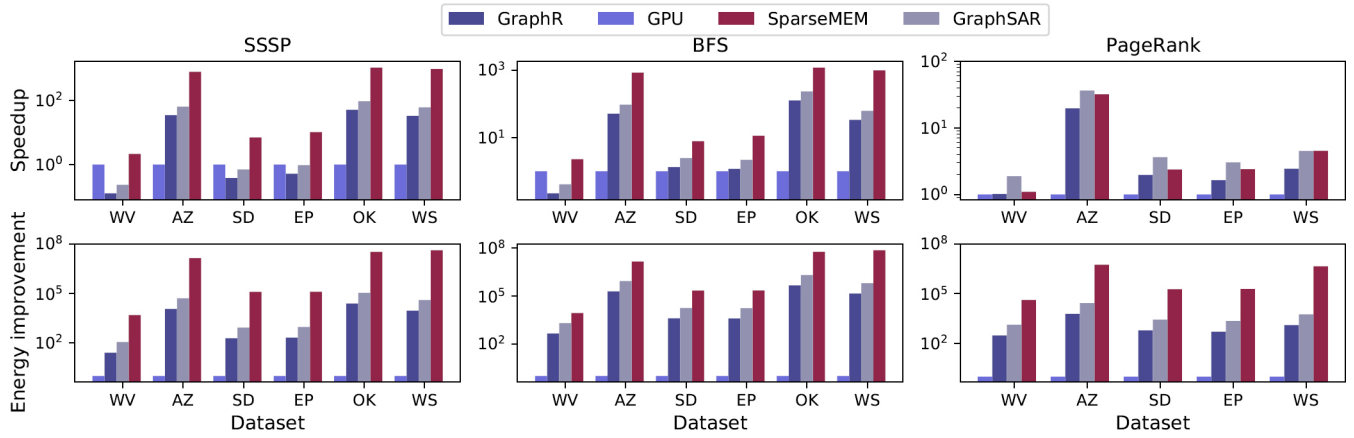
Fig. 7: Speedup and energy improvement of SparseMEM compared to the baselines for three algorithms (normalized to GPU)
