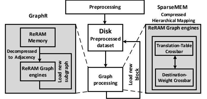
Fig. 3: SparseMEM and GraphR workflow comparison. Reducing the overhead of device programming by enabling computation over a compressed representation
