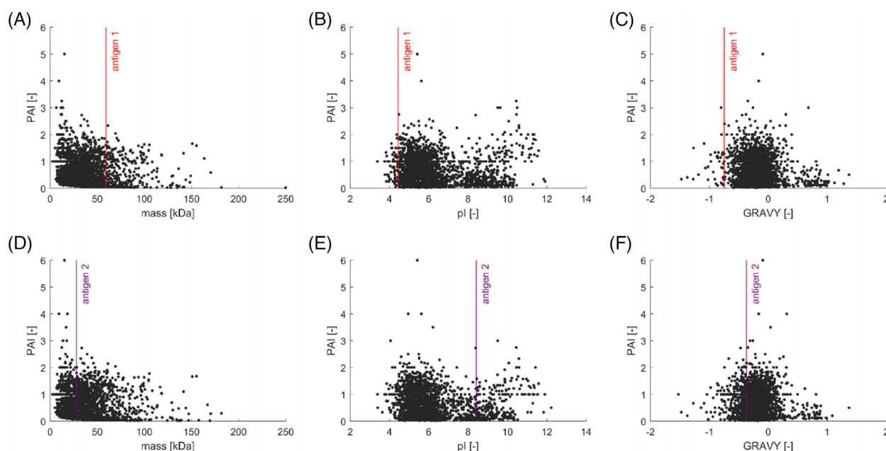
FIGURE 3 Abundances of the detected HCPs from null plasmid fermentations of the E. coli strains BLR (A–C) and HMS174 (D–F) are compared: (A and D) the mass of the proteins according to mass spectrometric measurements, (B and E) the average predicted isoelectric points (pI), and (C and F) hydrophobicity (GRAVY). Positive and negative GRAVY values describe hydrophobic and hydrophilic proteins, respectively. The model antigens 1 and 2 are indicated in red and purple. The abundances are expressed by the PAI parameter.
