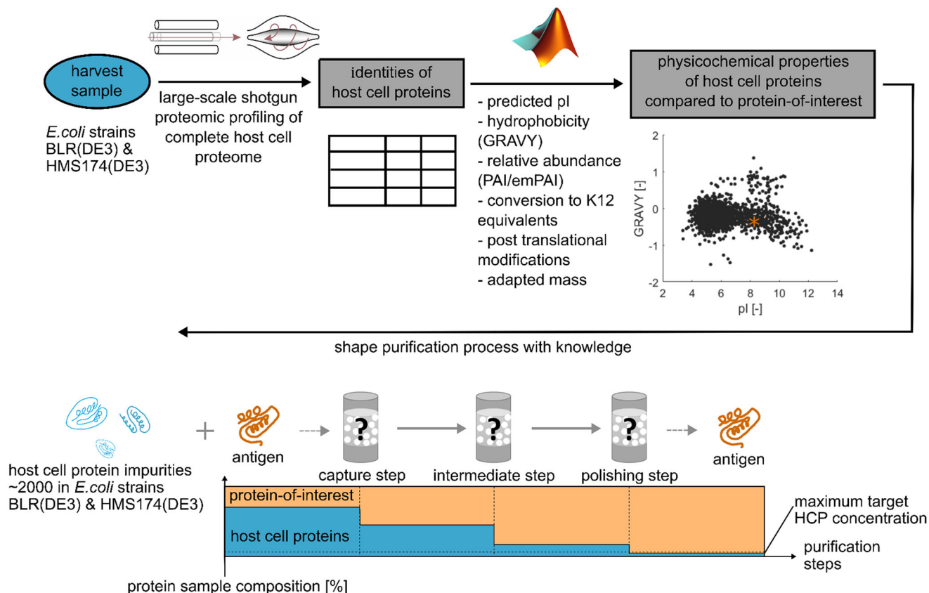
FIGURE 1 Schematic overview of the process development approach guided by large-scale host cell proteomics described in this study. The clarified harvest sample from the fermentation process was analysed using mass-spectrometry-based proteomics to identify all detectable HCPs. Further, a range of physicochemical properties was calculated for every possible gene product. One can guide the selection of the most suitable purification process by comparing the properties of protein therapeutics with those in the established database resource.
