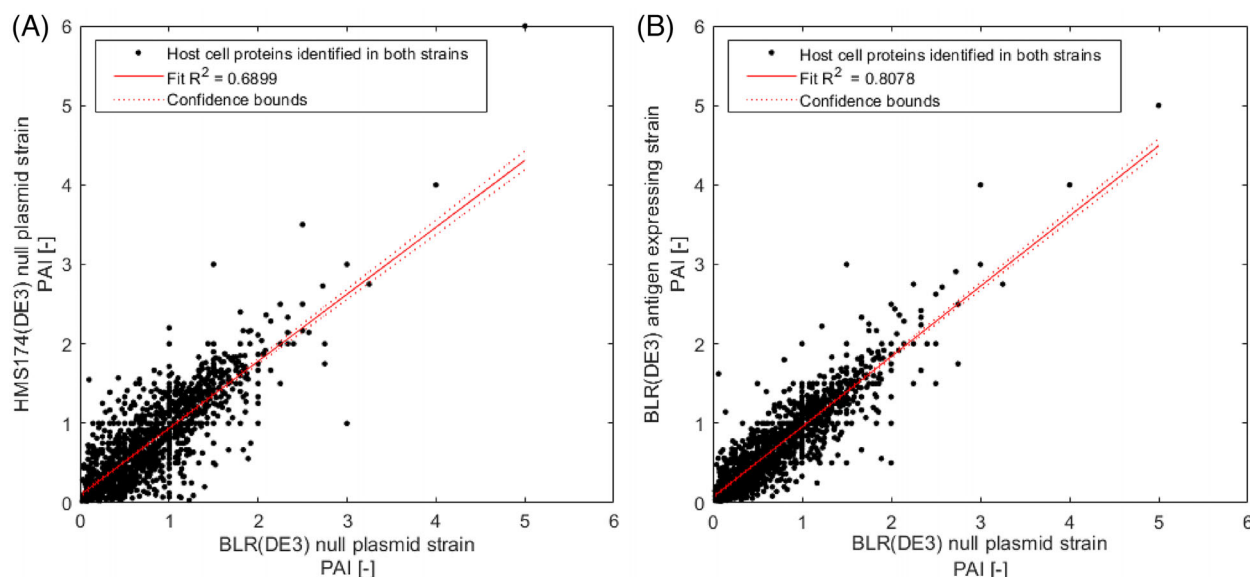
FIGURE 2 Scatterplots of the HCPs identified in the investigated E. coli strains. (A) presents a comparison of null plasmid E. coli strains BLR and HMS174. The correlation of 1590 proteins that were common to both strains resulted in an R^2 value of 0.6899. In (B), the null plasmid BLR was compared to the corresponding antigen-expressing strain; 1779 proteins were common to both samples, resulting in an R^2 value of 0.8078.
