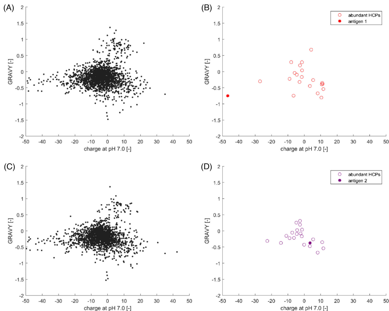
FIGURE 5 Comparison of HCPs from the null plasmid fermentations of the E. coli strains BLR (A and B) and HMS174 (C and D). The predicted hydrophobicity (GRAVY) is plotted against the predicted net charge at pH 7.0. Displayed are (A) the properties of the complete, identified host cell proteome of BLR; (B) the properties of the most abundant HCPs and antigen 1 in BLR; (C) the properties of the complete, identified host cell proteome of HMS174; and (D) the properties of the most abundant HCPs and antigen 2 in HMS174.
