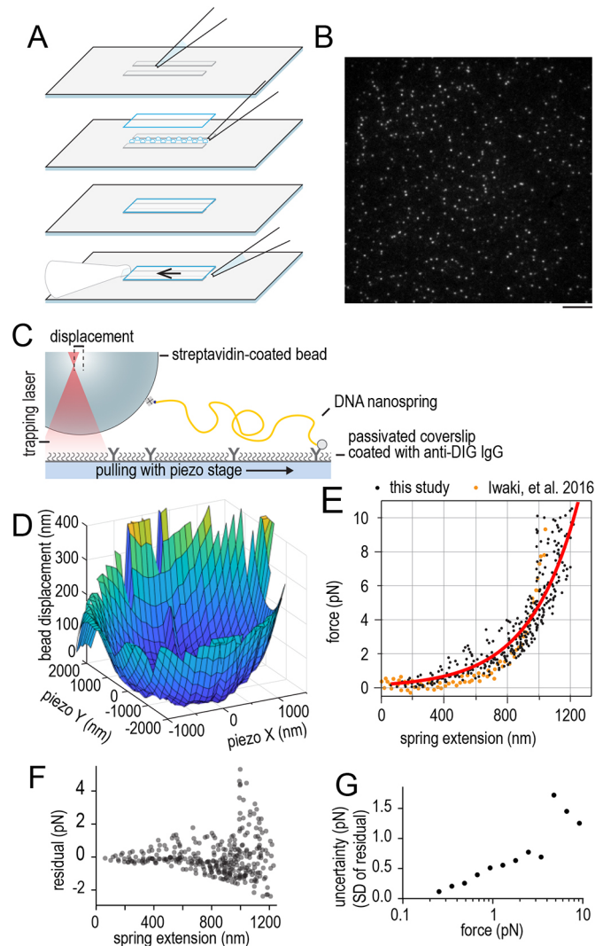
Fig. 2. Surface attachment and calibration of nanospring force–extension. (A) Schematic diagram showing assembly of a flow chamber using silanized slides and coverslips. (B) Typical microscopic field of view with 10× Atto-labelled nanosprings attached to glass surface using DIG and anti-DIG IgG. Scale bar: 10 μm. (C) Schematic diagram of an experiment with surface-bound nanospring being stretched using a bead in an optical trap. (D) A typical result (from six repeats) showing nanospring extension (vertical axis) as a function of the 2D coordinates of the microscopic stage (horizontal axes x and y ). The bell-like shape of the curve signifies a single attachment point for the nanospring. (E) Force–extension curve resulting from measurements using six nanospring-attached beads (black), overlaid on top of the results presented in the original publication (orange; Iwaki et al., 2016). Solid red line shows results of exponential fitting. (F) Residuals of exponential fitting presented in E. (G) Standard deviation of residuals binned by force (as calculated from spring extension).
