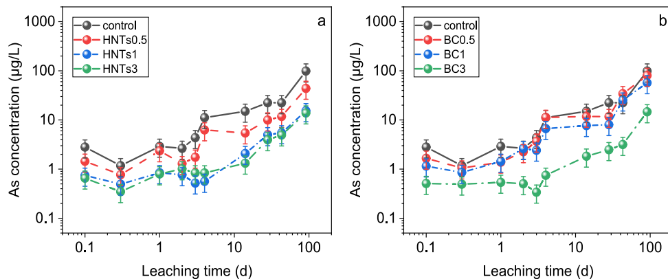
Fig. 6. The influence of HNTs and BC on the As leaching concentration from BAW with time: the influence of HNTs (a) and BC (b).
