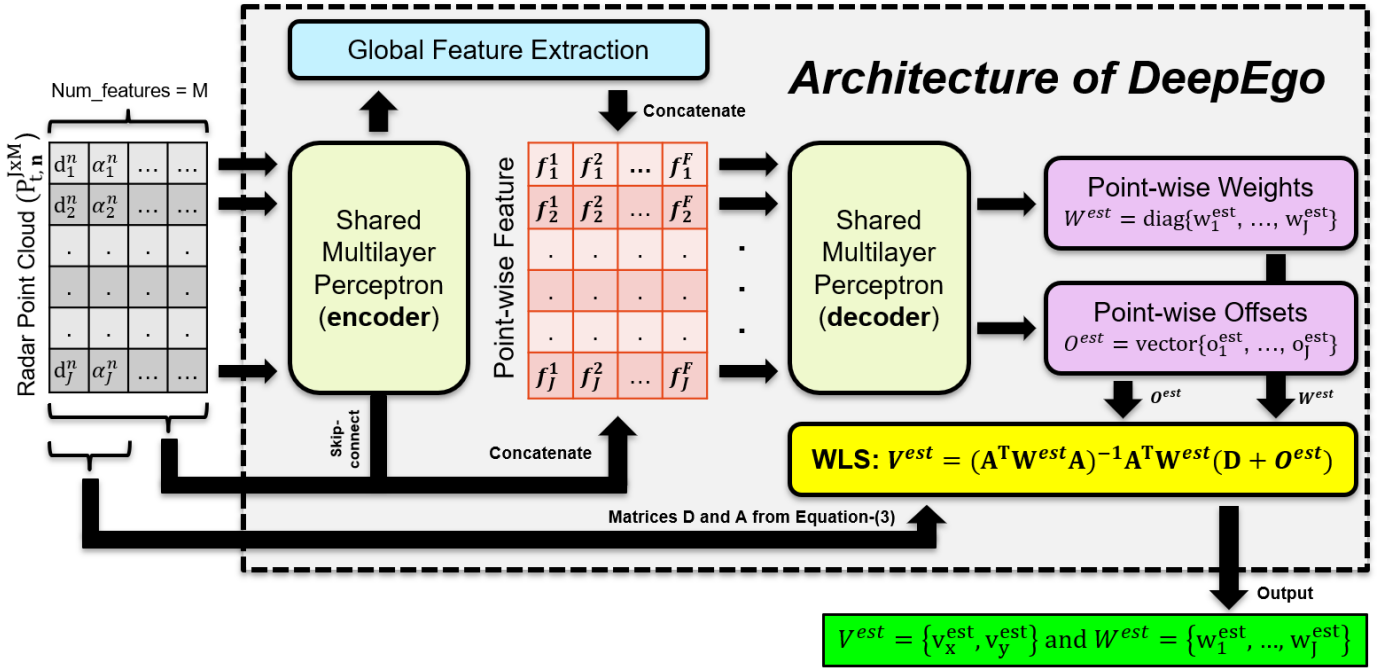
Fig. 1. The architecture of the proposed method (DeepEgo). The input data is the radar point cloud with J number of points and M number of features. Note that M \geq 2 is required in this work because radial velocity and AoA measurements are essential object features for instantaneous ego-motion estimation. The outputs of DeepEgo are the motion predictions V^{est} and pointwise weights W^{est} .
