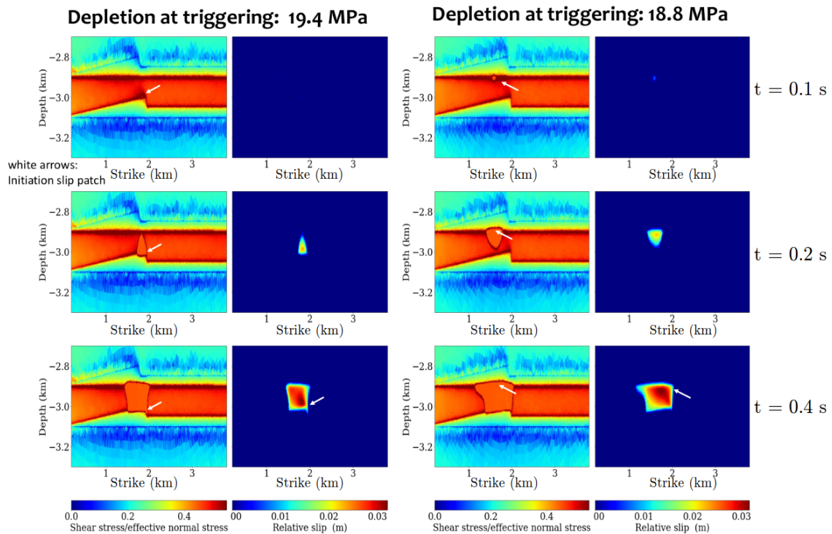
Figure 2 Results of dynamic simulation of seismic events showing the stress field and the displacement. Left: the model with 30° intersection angle. Right: the model with 60° intersection angle.
