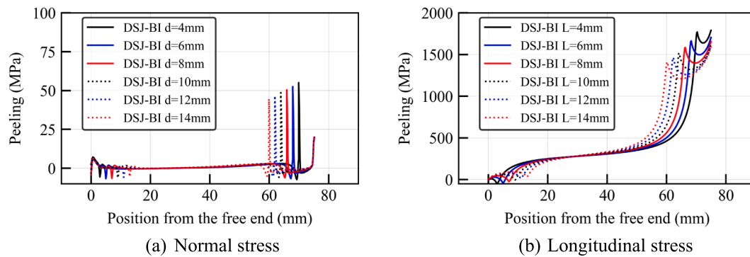
Fig. 22. Comparison between the stress distribution obtained numerically along the path shown in Fig. 19 for DSJ-BI with different ductile adhesive length.
