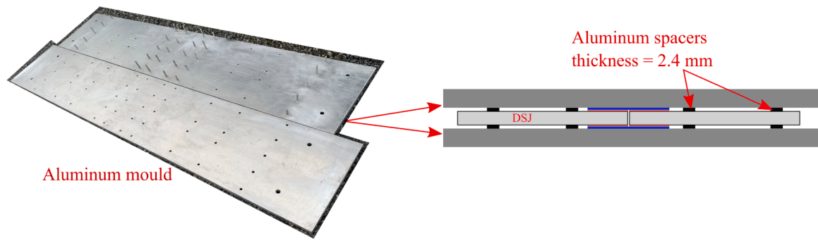
Fig. 3. Aluminium mould for the fabrication of DSJ specimens.
