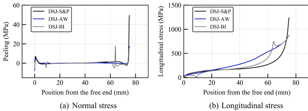
Fig. 21. Comparison between the stress distribution obtained numerically along the path shown in Fig. 18 for DSJ-S&P, DSJ-AW, and DSJ-BI.
