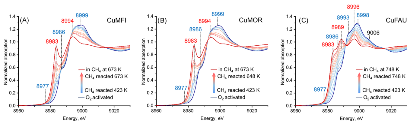
Figure 2. XANES spectra acquired at different stages of the reaction between CuMFI (A), CuMOR (B), and CuFAU (C) and methane. Labels of the signals corresponding to \text{Cu}^{\text{II}} and \text{Cu}^{\text{I}} species are colored in blue and red, respectively. The spectra shown in blue thick lines correspond to oxygen-activated materials and are acquired at ambient temperature, the spectra shown in thin lines are related to the state of the materials after the reaction with methane at various temperature and are acquired at ambient temperature, and the spectra shown in red thick lines correspond to the highest reaction temperature with acquisition exactly at the corresponding temperature without cooling.
