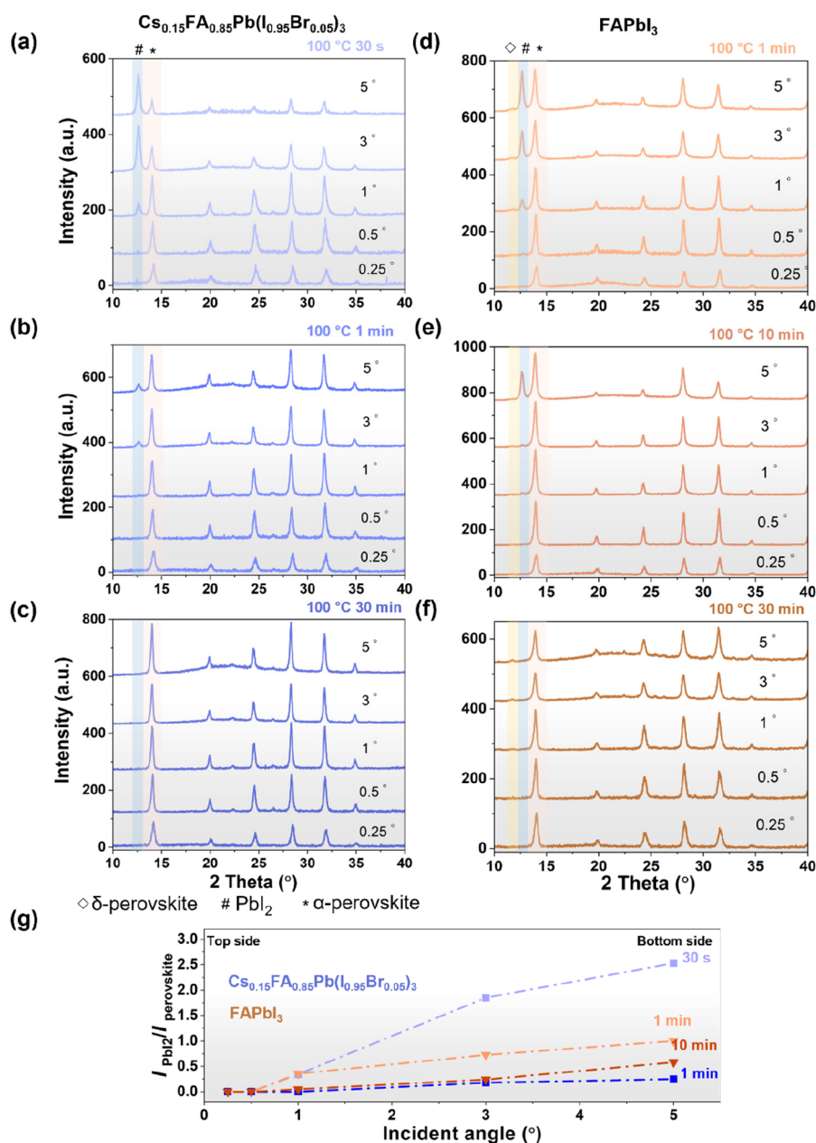
Figure 4. (a–c) GIXRD measurements on 400 nm thick \text{CsFAPbI}_3\text{Br} films with different annealing times: (a) 30 s, (b) 1 min, and (c) 30 min. (d–f) GIXRD measurements on 400 nm thick \text{FAPbI}_3 with different annealing times: (d) 1 min, (e) 10 min, and (f) 30 min. The \delta -phase PVK peak is highlighted in yellow; the \text{PbI}_2 (100) peak is highlighted in light blue; and the PVK (100) peak is highlighted in light brown. (g) Dependence of the I_{\text{PbI}_2}/I_{\text{PVK}} (100) ratio extracted from Figure 4(a–f) as a function of incident angle for \text{CsFAPbI}_3\text{Br} and \text{FAPbI}_3 at different annealing times.
