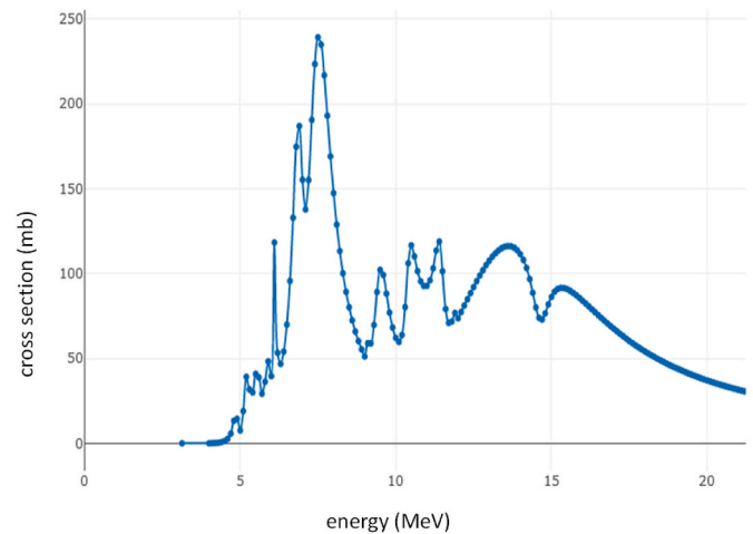
Fig. 2. Production cross section for ^{14}\text{N}(\text{p},\alpha)^{11}\text{C} . Data from (IAEA, 2022).
