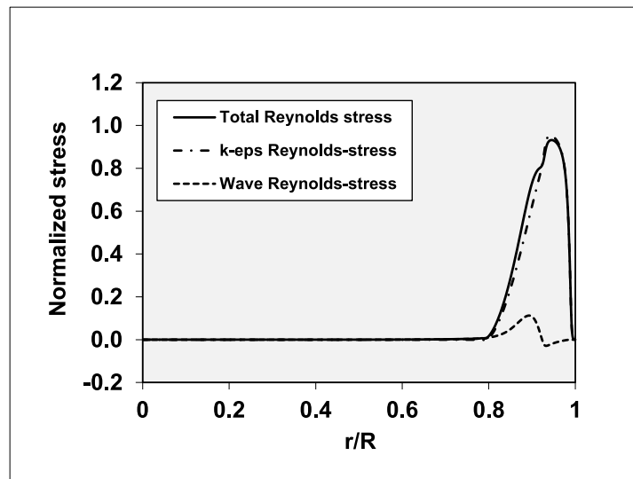
Fig. 16. Radial profile of the composition of the Reynolds stress in the RANS simulation for a water hold-up fraction \alpha_w = 0.29 and an imposed frictional pressure drop of 400 Pa/m.
