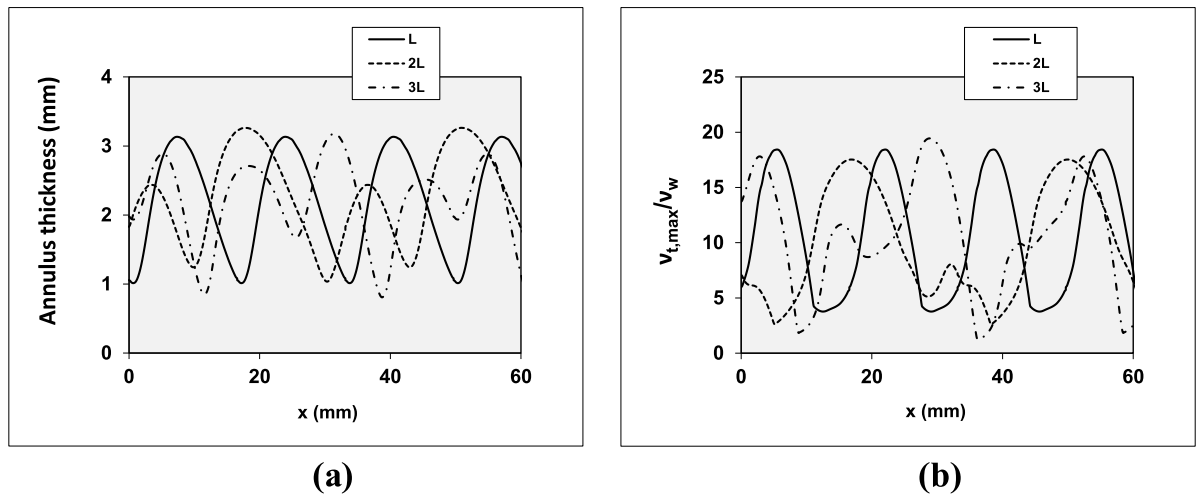
Fig. 6. RANS results with different pipe section lengths (values shown in legend, L=16.6 mm) for (a) annulus thickness, and (b) maximum turbulent viscosity; water hold-up fraction \alpha_w=0.29 , oil viscosity is \mu_o=0.75 Pa s, frictional pressure drop is 400 Pa/m.
