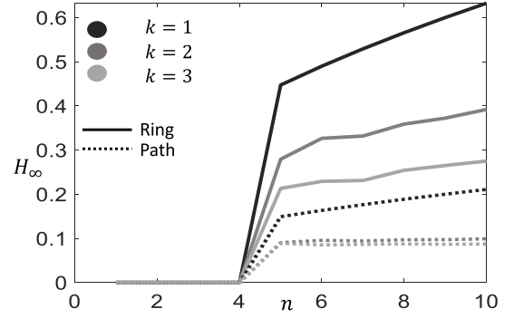
Fig. 8. \mathcal{H}_\infty norm for unidirectional ring and line topologies.
