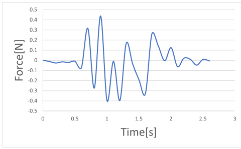
Fig. 14. Reaction force for unbalanced manipulator in the X direction for the experiment when the platform is moved up such that \phi_{1i} = 40^\circ, i \in 1, 2, 3 , from its resting position (lowest potential)
