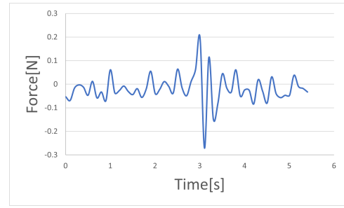
Fig. 16. Reaction forces in the case of an balanced manipulator in the X direction for the experiment when the platform is moved forward and back in the X direction. The motion is such that \phi_{11} = 40^\circ in the middle of the cycle.
