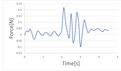
Fig. 17. Reaction force for balanced manipulator in the X direction for the experiment when the platform is moved up such that \phi_{1i} = 40^\circ, i \in 1, 2, 3 , from the same position as the resting position of the unbalanced case
