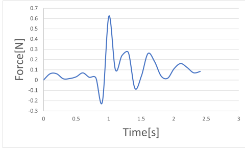
Fig. 15. Reaction forces in the case of an unbalanced manipulator in the X direction for the experiment when the platform is moved forward and back in the X direction. The motion is such that \phi_{11} = 40^\circ in the middle of the cycle.
