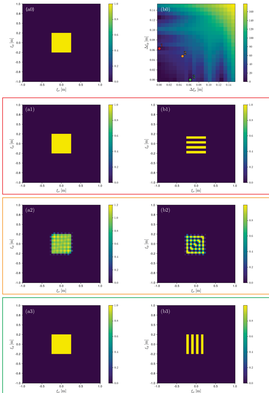
Fig. 7. (a0) Desired irradiance distribution: square distribution of width 0.5; (b0) loss landscape. (a1), (b1) Total irradiance and impulse response obtained for \Delta\boldsymbol{\xi} = (0, 8\Delta\xi_y) (red dot). (a2), (b2) Total irradiance and impulse response obtained for \Delta\boldsymbol{\xi} = (6\Delta\xi_x, 6\Delta\xi_y) (orange dot). (a3), (b3) Total irradiance and impulse response obtained for \Delta\boldsymbol{\xi} = (8\Delta\xi_x, 0) (green dot).
