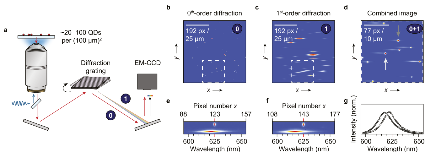
Figure 1. Multiparticle spectroscopy. (a) Luminescence from 20 to 100 QDs is collected simultaneously by a microscope objective. The image is directed to the entrance of a spectrometer (without the use of a slit) equipped with a diffraction grating. By positioning the grating at different angles, we project either the 0th-order reflection image (0) or the 1st-order diffraction image (1) onto a pixel-array camera. (b) Image of the 0th-order diffraction of a field of view containing several tens of CdSe/CdS/ZnS QDs. (c) The corresponding image of the dispersed 1st-order diffraction. The horizontally elongated emission spots contain spectral information. (d) Overlay of the 0th-order and 1st-order diffraction images. (e, f) Zoom-in views of the 0th-order and 1st-order diffraction images of the QDs highlighted in (d) (vertically offset for clarity). To obtain emission spectra, the wavelength axis is calibrated by fixing a center wavelength (625 nm in this experiment, approximately at the ensemble emission peak) at the pixel number x that corresponds to the center of the emission spot in the 0th-order diffraction image. (g) Resulting single-QD emission spectra of the two CdSe/CdS/ZnS QDs highlighted in (d).
