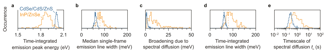
Figure 3. Variations in single-particle emission properties within batches of QDs. (a) Distribution of the time-integrated emission energy, (b) single-frame emission line width, and (c) spectral diffusion-induced broadening. (d) As a result of spectral diffusion, the time-integrated emission line width is broadened with respect to the single-frame line width. (e) Histograms of the relevant time scales associated with SD. Results are shown for 491 CdSe/CdS/ZnS and 154 InP/ZnSe QDs (blue and yellow histograms, respectively).
