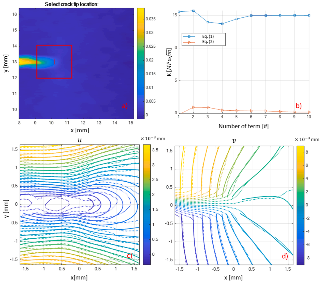
Fig. 7. Schematic of field fitting approach to extract stress intensity factor values, (a) crack tip selection, (b) optimised stress intensity, and (c) & (d) resulting field fits.
