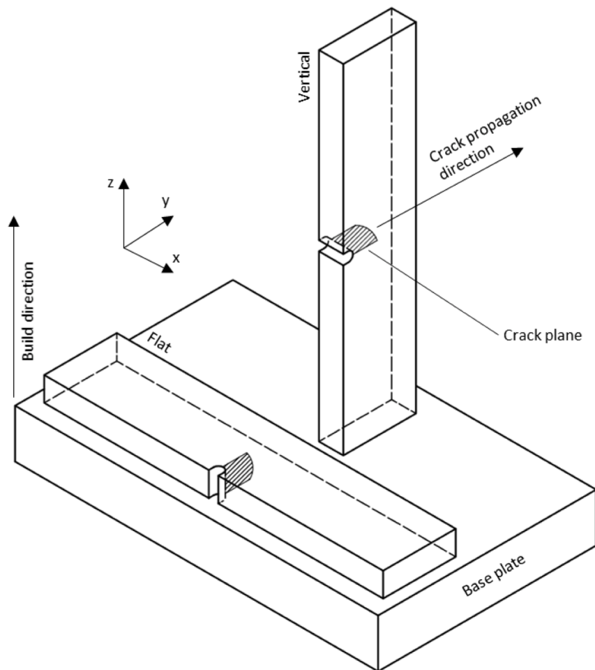
Fig. 1. Specimen build orientations, crack planes and crack propagation direction.
