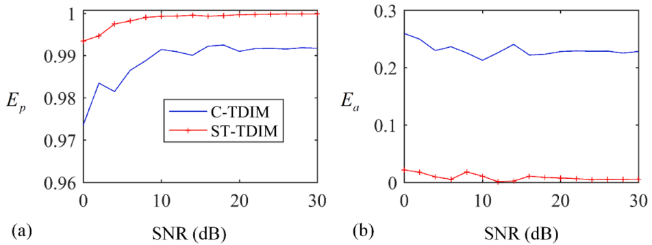
Fig. 10. The phase indicators E_p (a) and the amplitude indicators E_a (b) of the unsteady rotating forces at different SNRs when 48 sampling points are used.
