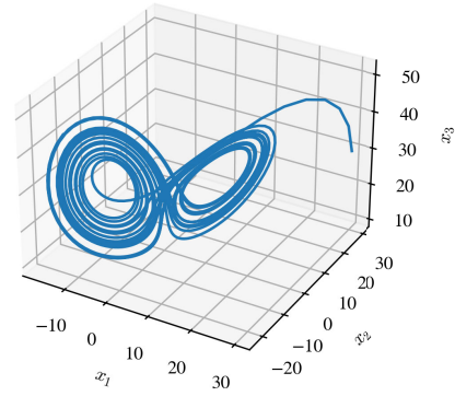
FIGURE 7. Open-loop Lorenz system trajectory.
