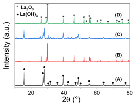
Figure D1: XRD profile of \text{La}_2\text{O}_3 sample with different treatment: (a) directly purchased \text{La}_2\text{O}_3 ; (b) after calcining (a) at 700 °C in air for 5 h; (c) after keeping (b) in a closed sample vial at room temperature for 1 day; (d) after calcine (a) in 50 vol% \text{O}_2 in He (50 mL/min) at 700 °C for 30 min.
