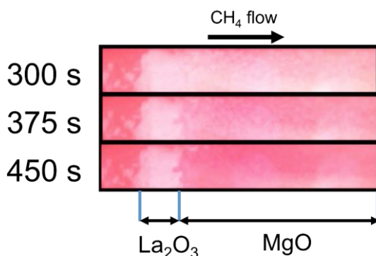
Figure D2: Operando visualisation of \text{La}_2\text{O}_3 -MgO mixed catalytic bed ( \text{La}_2\text{O}_3 10 wt% at the front part of the catalytic bed) during \text{CH}_4 pulse in unsteady-state OCM reaction at 900 °C.
