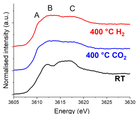
Figure A3: In situ potassium K-edge XANES of Cu-K/Al 2 O 3 catalyst (Cu 11 wt%, K 10 wt%) at room temperature (RT) and in reaction conditions averaged during 5 h at 400 °C in H 2 (10% in He) and 4 h at 400 °C in CO 2 (1 % in He).
