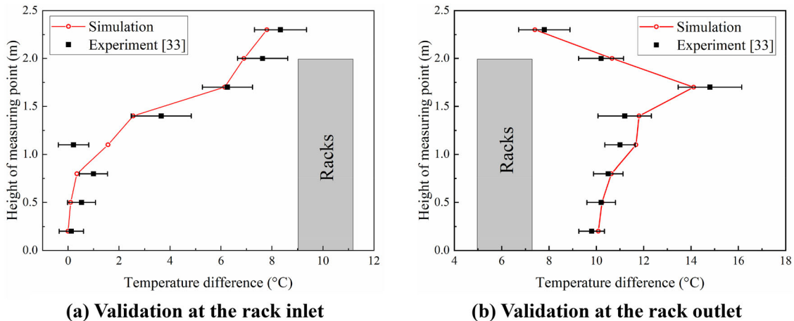
Figure 5. Model validation results at the rack inlet and outlet.
