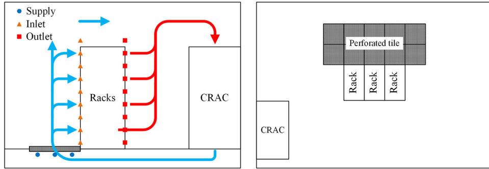
Figure 4. Experimental model arrangement in reference [33].
