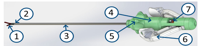
FIGURE 6. Compliant instrument design overview, with grasper tip (1), tip locking mechanism (2), shaft (3), balancing mechanism housing (4), rotating interface (5), handle (6) and push pull rod locking (7). Note that the used colors do not represent the final prototype.
