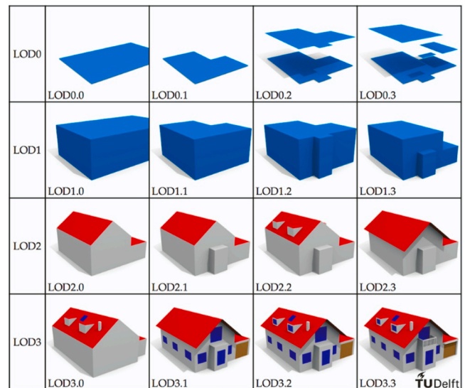
Fig. 4. The visualisation of improved LOD specification for 3D building models (Biljecki et al., 2016).
